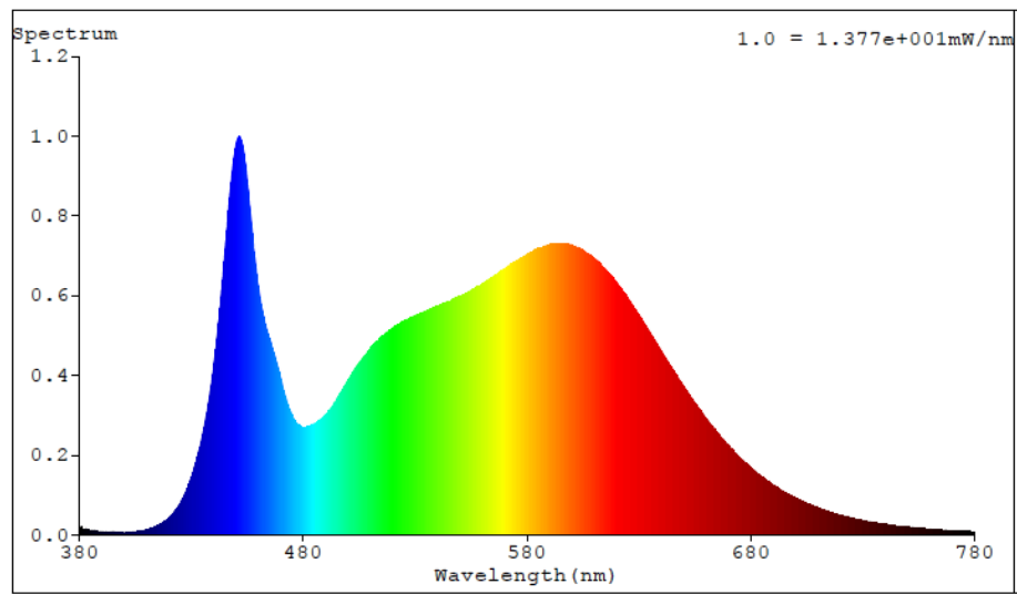
Spectral Distribution
